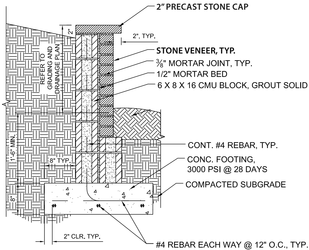
○ RETAINING WALL WITH VENEER
